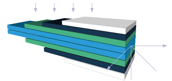
CFRP/GFRP laminate lay-up
